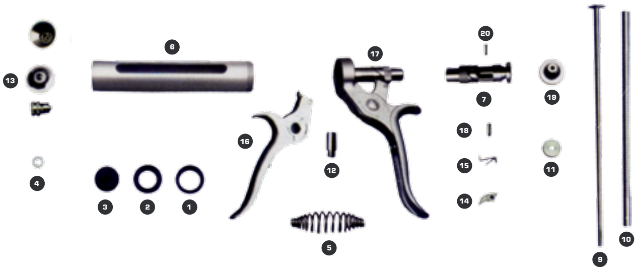
Ref. 250607 Alargadera Hauptner
